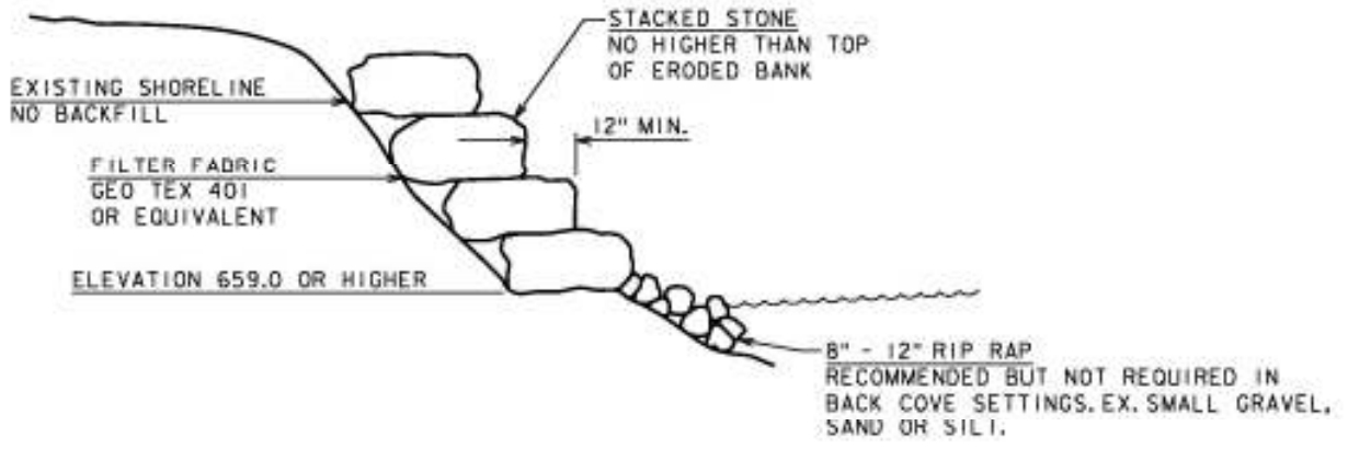
INSTALLATION OF RIP RAP / STACKED STONE
