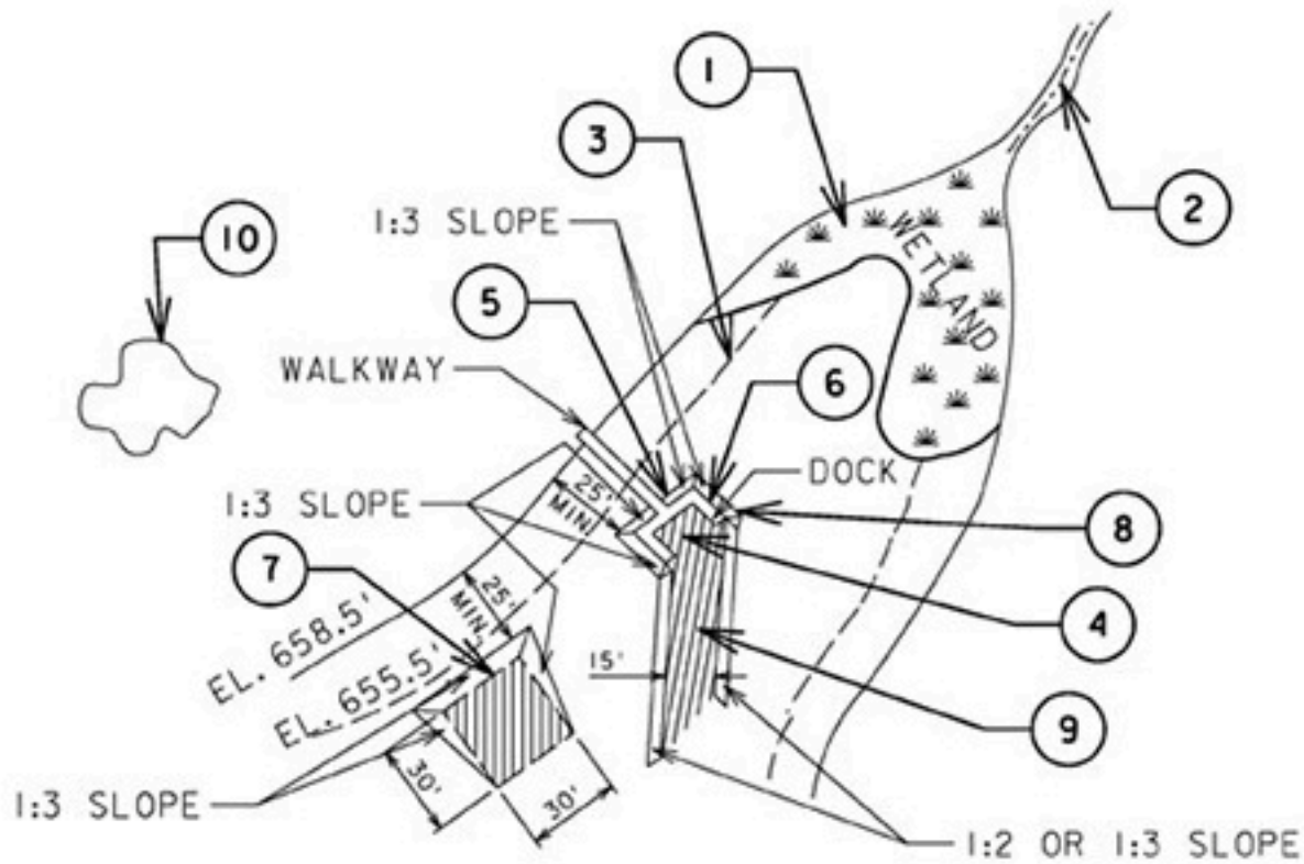
PLAN VIEW OF MINOR EXCAVATION
